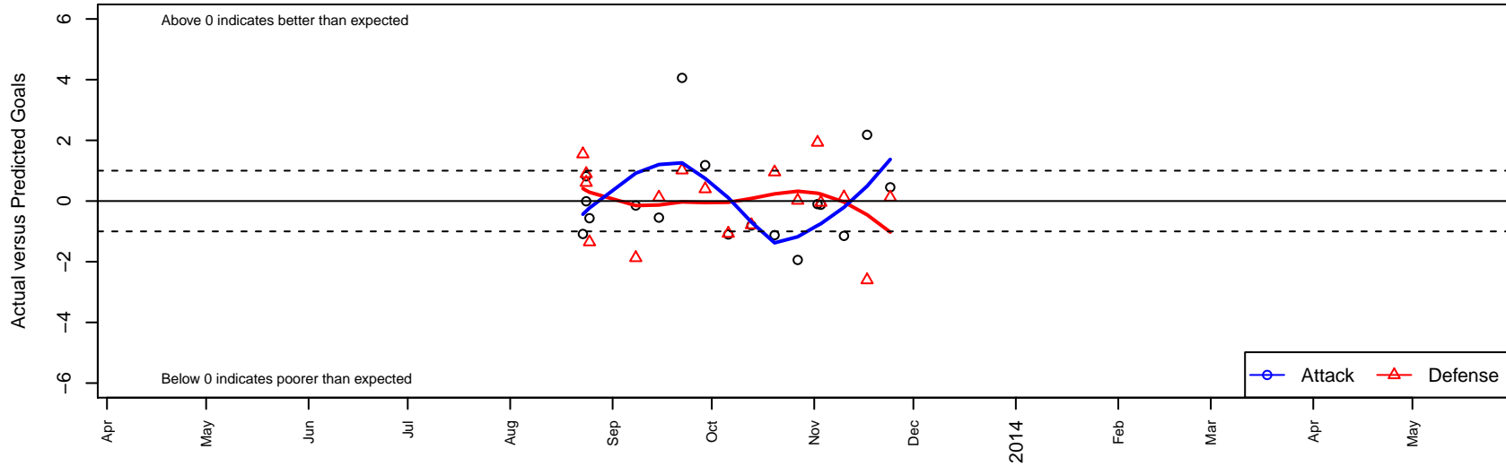
3 Rivers Black B95 Dots are actual minus expected GF (blue circles) and GA (red triangles). Blue line is smoothed change in attack strength. Red is smoothed change in defense strength.
